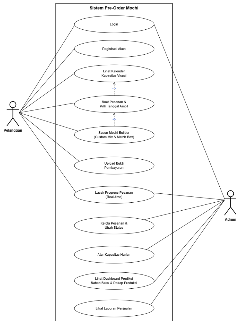
Gambar 1. Use Case Diagram Sistem Pre-Order Mochi
